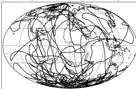
Fig. 5. Mollweide projection for VGP wander
