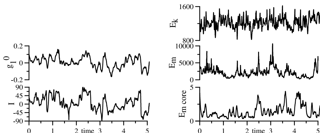
Fig. 6. Regime II, E = 3 \cdot 10^{-3} , Pr = 1 , Ra = 10^3 , q = 4 . Evolution of: magnetic dipole g_1^0 , inclination I , kinetic energy E_k , magnetic energy E_m , and magnetic energy of the inner core E_{m\_core}
